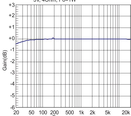
Frequency Response 5V, 40Ω
